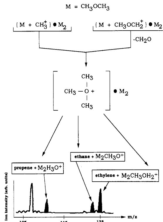
Figure 6. Proposed reaction mechanism for observed cluster ions generated through a common trimethyloxonium intermediate. Mass spectrum at bottom is for neat dimethyl ether cluster at 70 eV from dimer to trimer ( 80 – 140 amu). Major ion peaks are identified by their empirical formulas ( M = (CH_3)_2O ).
