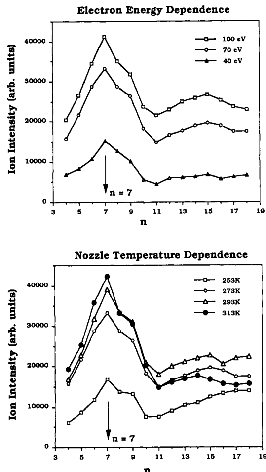
Figure 2. Intensity of \{\text{NH}_3\}_{n-1}\text{NH}_2^+ vs cluster size, as a function of electron-impact energy ( T_0 = 273 K, P_0 = 1 atm) and as a function of stagnation temperature (70 eV, P_0 = 1 atm). Note the prominent magic number at n = 7 . Reprinted with permission from ref 28. Copyright 1989 American Institute of Physics.
