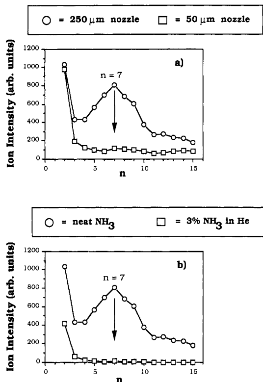
Figure 4. Ion intensity of [\text{NH}_3]_{n-1}\text{NH}_2^+ vs cluster size as a function of expansion conditions using 70-eV electron impact: (a) nozzle size (using neat ammonia); (b) expansion seeding (nozzle diameter = 250 \mu\text{m} ). Note the loss of the magic number at n = 7 occurring for expansion conditions which generate smaller clusters.
